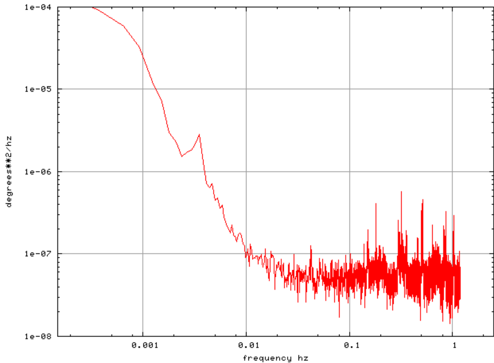
Lucas inclinometer - float: incl1 power spectrum
